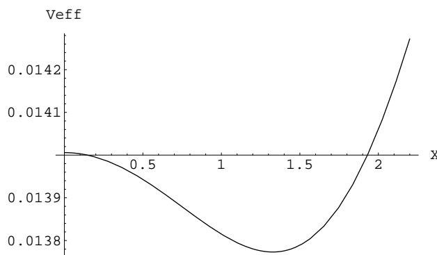
Figure 3: A plot of V_{\text{eff}}^{(1)} vs. |X| for the theory (3.1) with m_1 = 1, m_2 = 4, \lambda = 1, y = 0.2 . The R-breaking local minimum of the potential occurs at |X| \approx 1.3 . According to the bound (3.5), a transverse direction (a linear combination of the \phi_i fields) becomes tachyonic for |X| > 2.4 .
